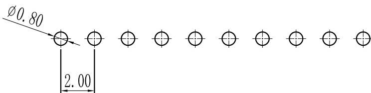
PCB LAYOUT
